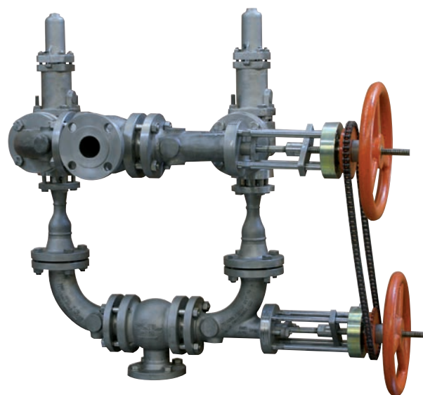
Tandem Changeover Valve – Model 69
