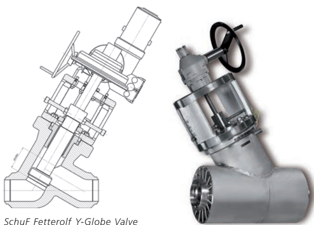
SchuF Fetterolf Y-Globe Valve
