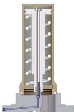
73IS Compact TESO design
