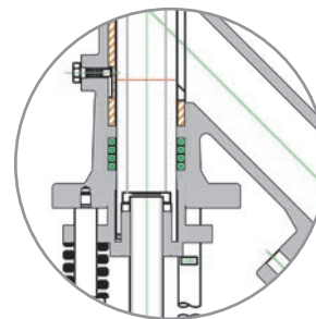
Detail: 26FR – Super Closure
