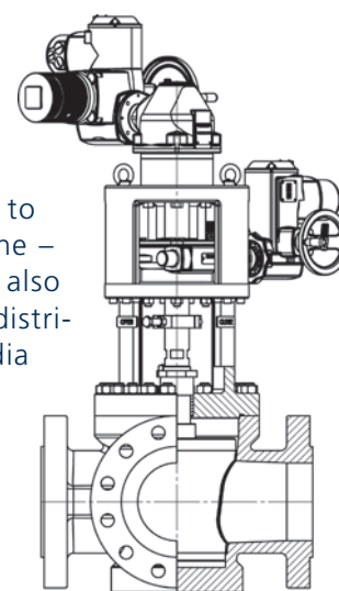
4-Way SwitchPlug Valve
