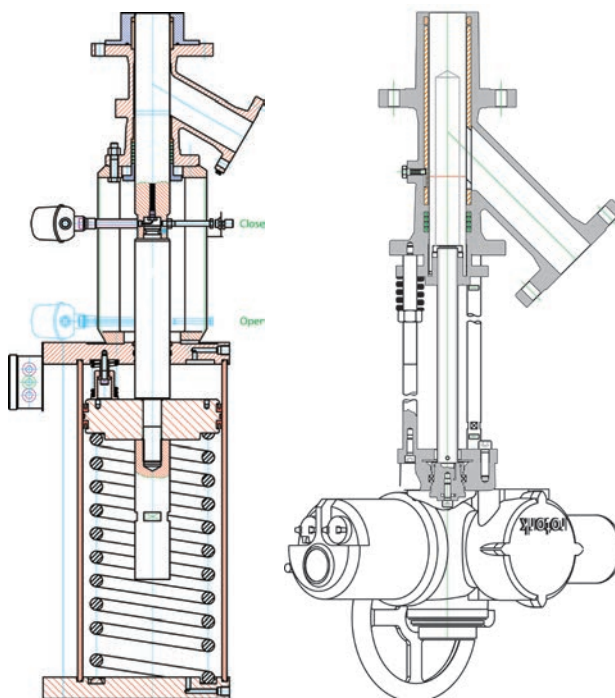
Ram drain valve – Model 28KR
