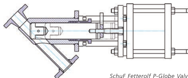
SchuF Fetterolf P-Globe Valve
