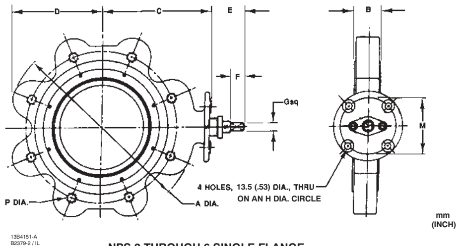
Figure 7. Dimensions and Weights Wafer and Single Flange Style CL600 (also see table 26)
