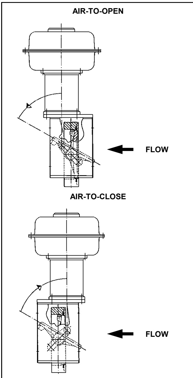
FIGURE 2 - DISC ROTATION
