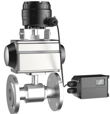
Ex ia remote rotary type
