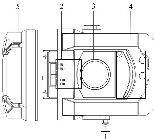
Ex d positioner structure
